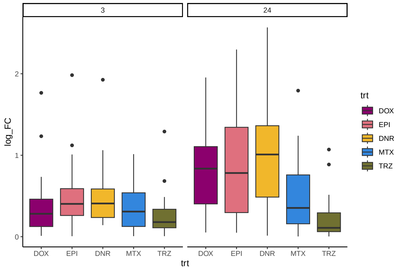
logFC of HF overlapping regions, n = 29
